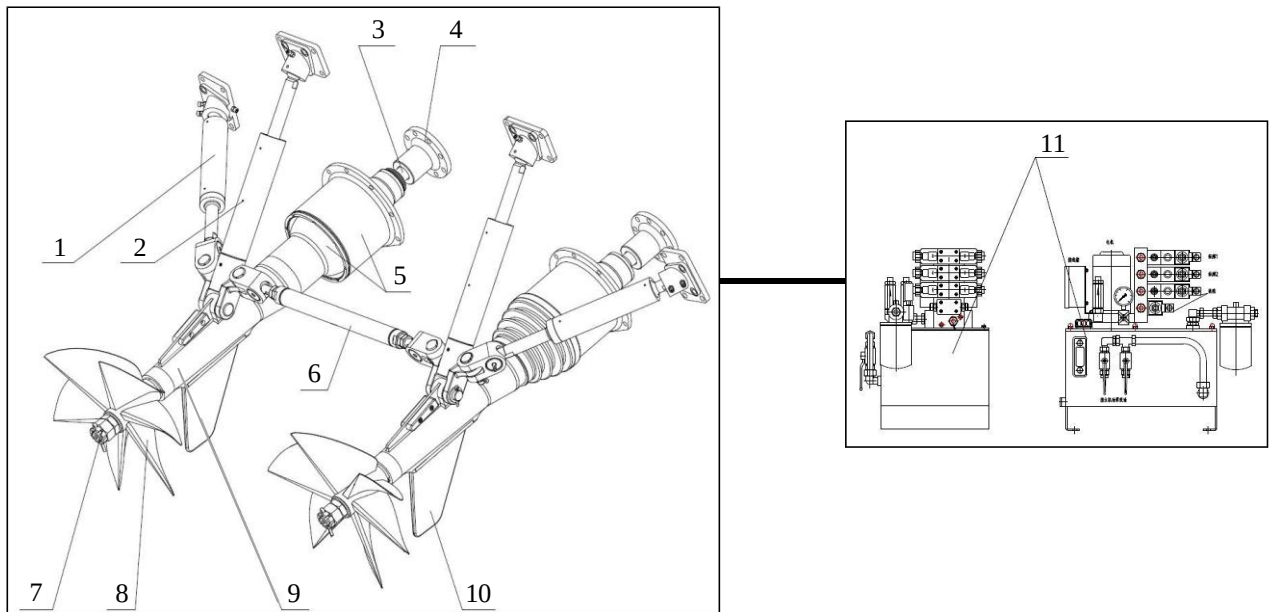
1 Steering cylinder 2 Trim cylinder 3 Input shaft 4 Flange coupling 5 Ball seat and sphere 6 Connecting rod 7 Propeller shaft 8 Propeller 9 Bracket 10 Rudder plate 11 Hydraulic power unit and control box
